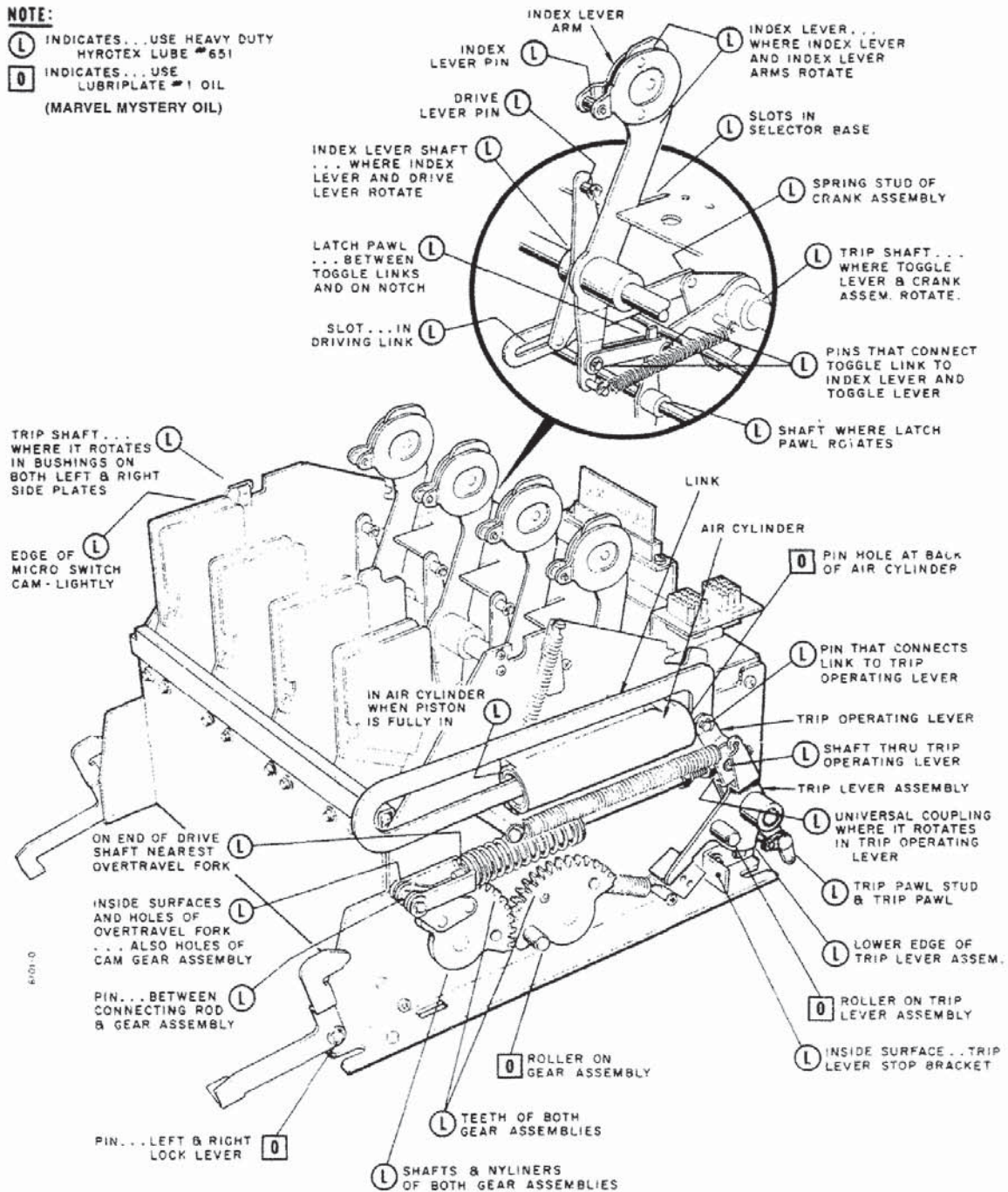
Figure 12. Reel Mechanism - (Soft Cushion)
